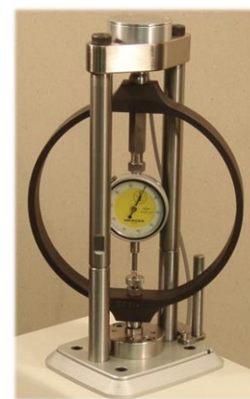
Calibration using a proving ring
